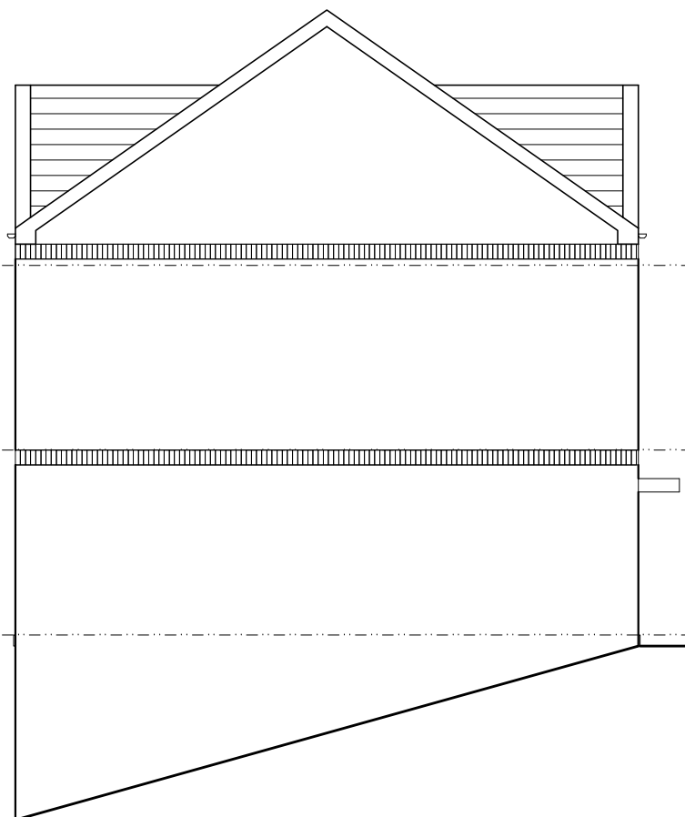
SIDE ELEVATION
