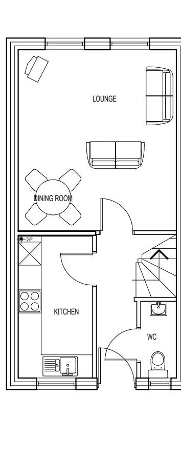
GROUND FLOOR PLAN AREA - 34.97sqm
