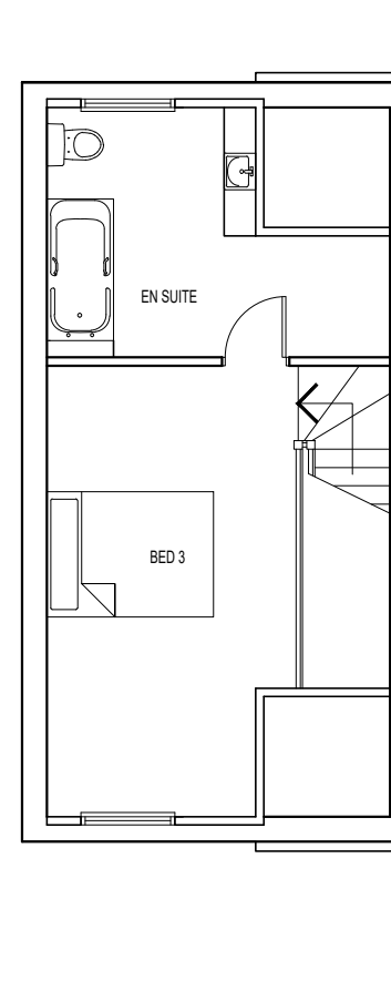
SECOND FLOOR PLAN AREA - 25.58sqm
