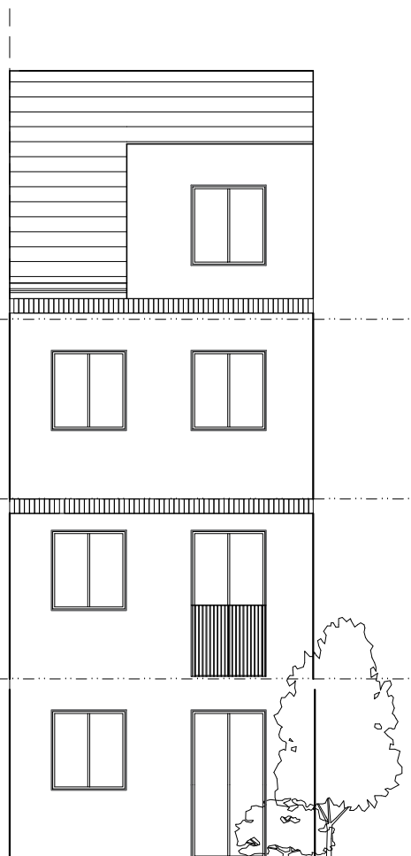
REAR ELEVATION
