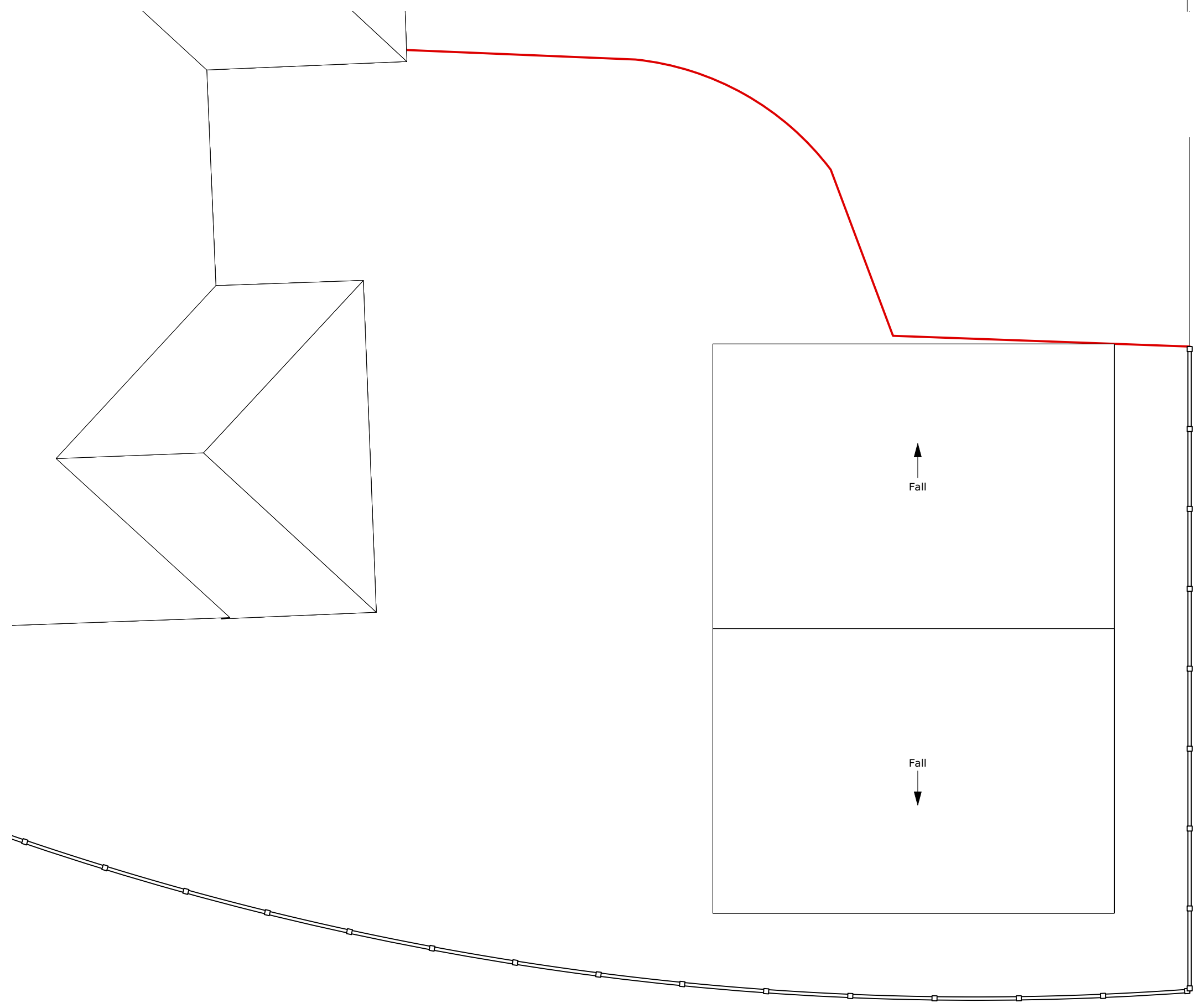
1 Proposed Garage Roof Plan Scale: 1:50
