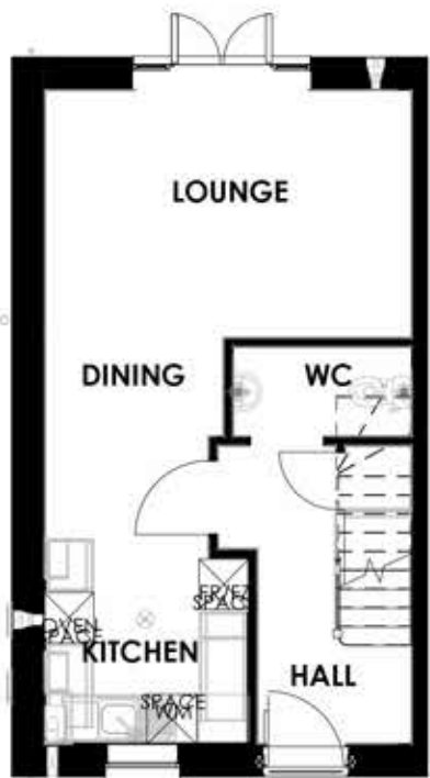
GROUND FLOOR 1 : 100
