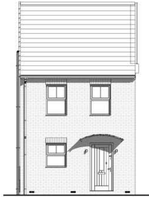
FRONT ELEVATION 1 : 100
