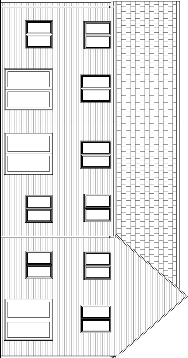
Rear Elevation
