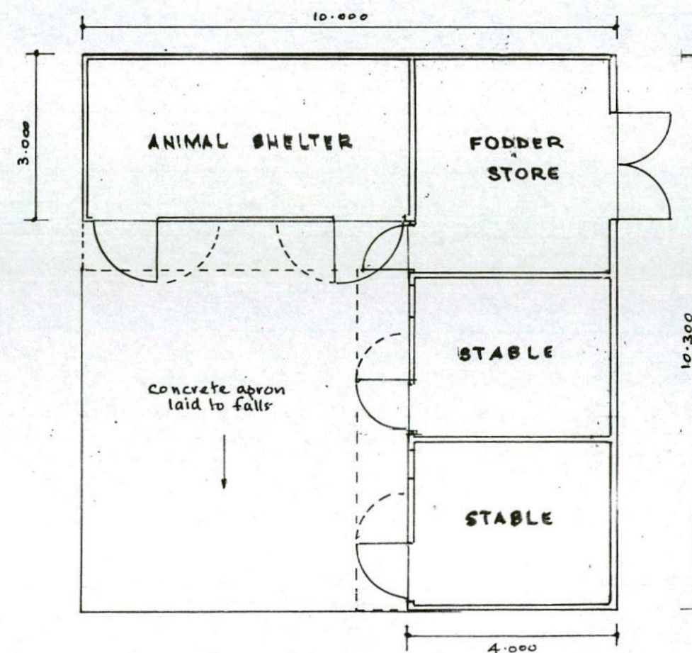
PLAN
