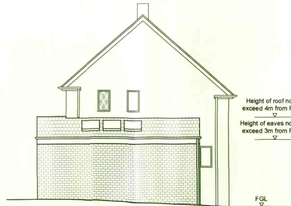
Side Elevation Proposed 1:100
