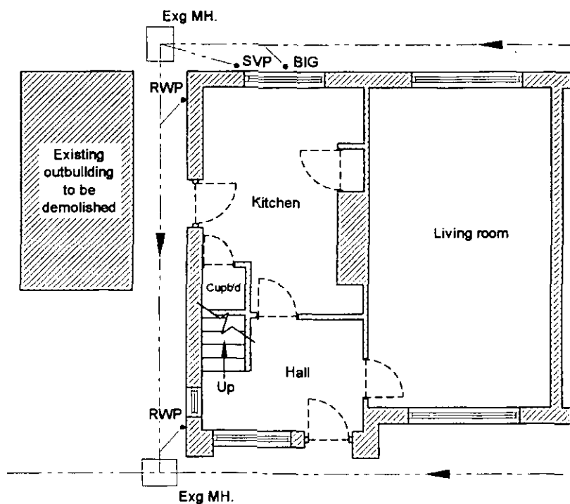
Ground Floor Existing 1:100
