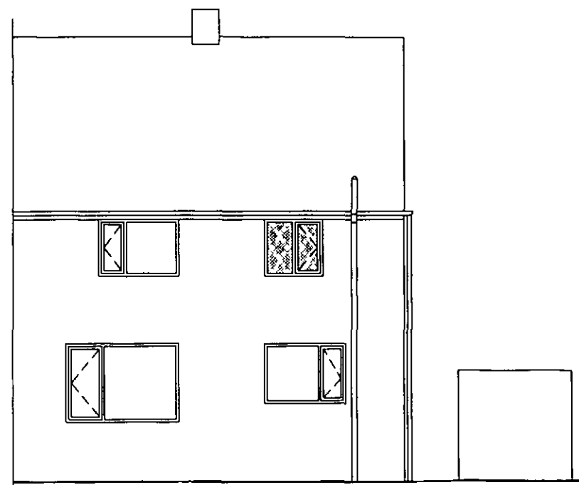
Rear Elevation Existing 1:100
