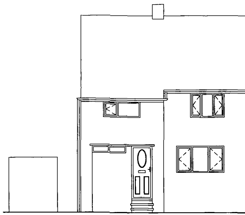
Front Elevation Existing 1:100
