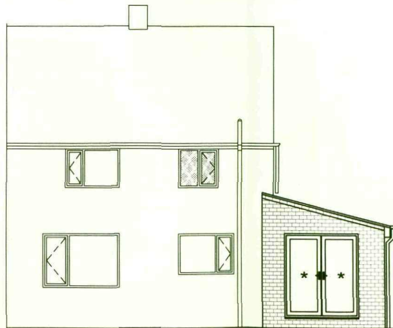
Rear Elevation Proposed 1:100
