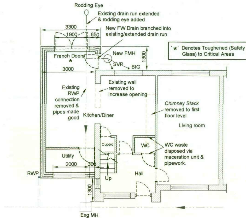
Ground Floor Proposed 1:100
