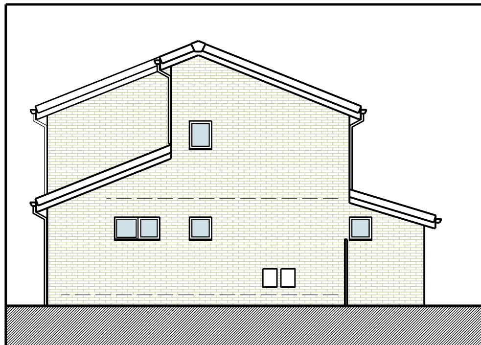
South Elevation
