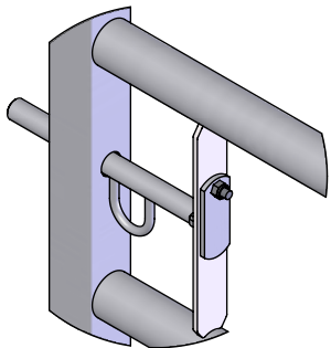
20 DIA. KEYHOLE / PENDULUM SLIDING BOLT DETAIL
