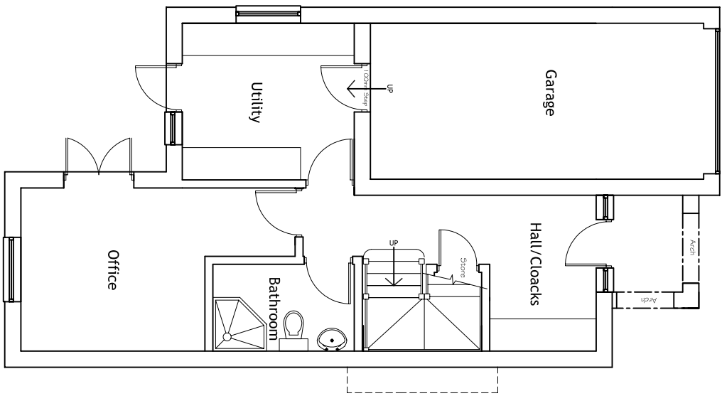
GROUND FLOOR PLAN 0 1m 2m 3m
