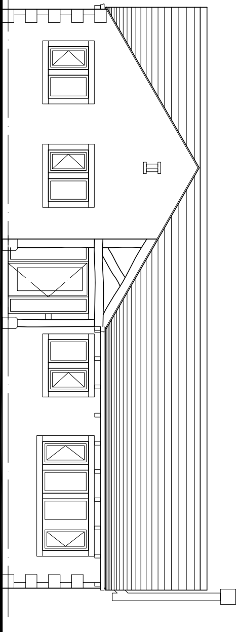
NORTH WEST ELEVATION (Front)
