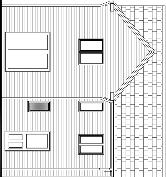
Rear Elevation
