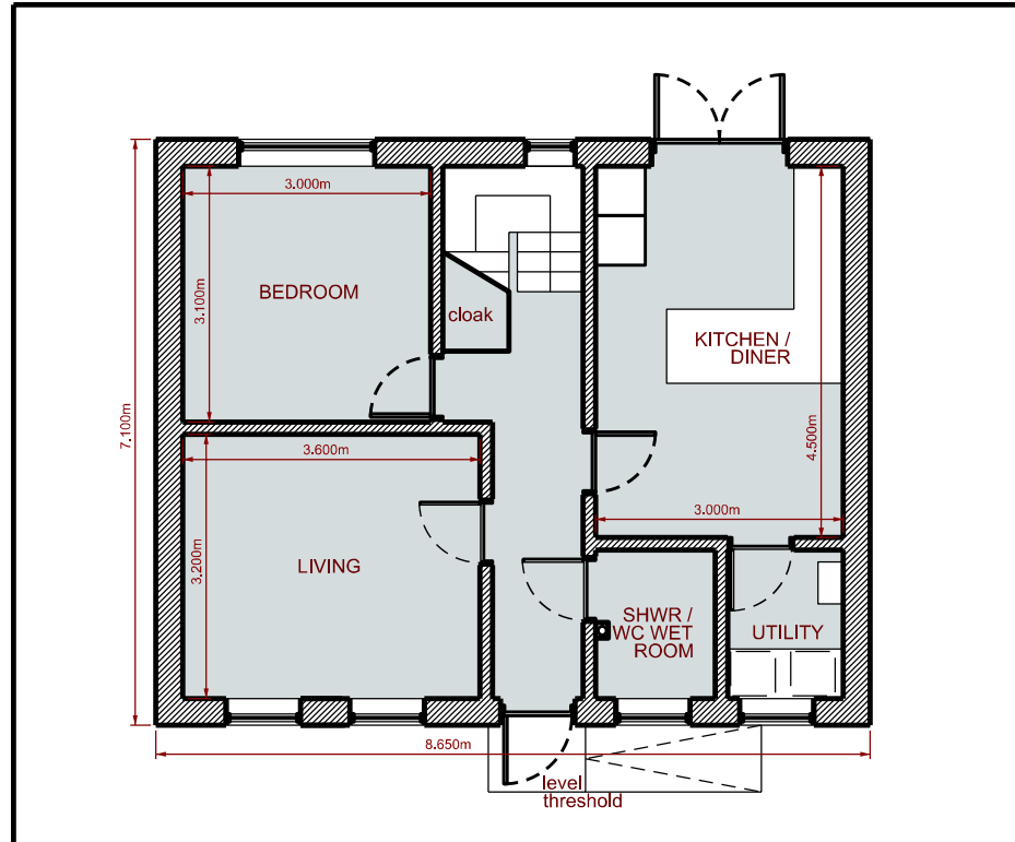
Ground Floor Plan - Proposed 1:100 No1,2,3,4
