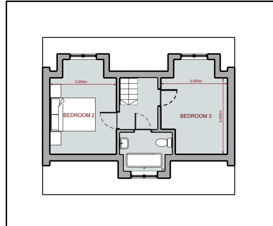
First Floor Plan - Proposed 1:100 No1,2,3,4
