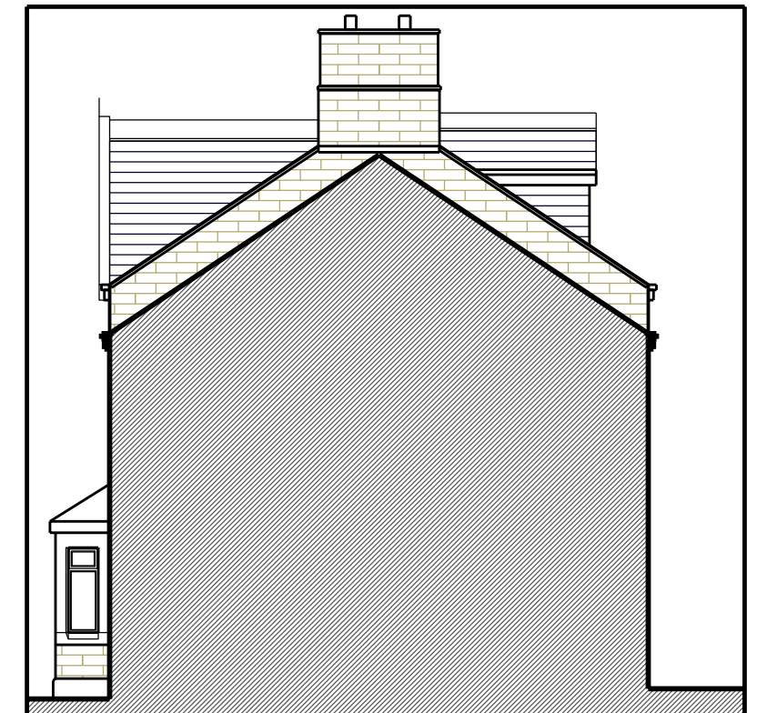
West Elevation - Proposed
