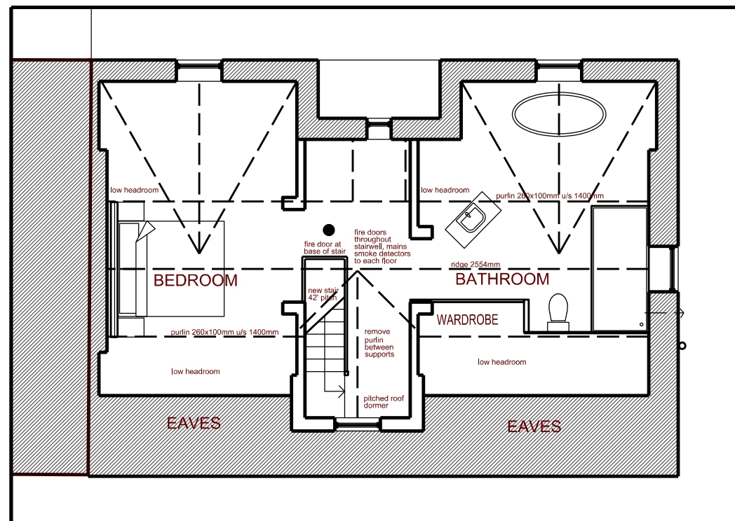
Second Floor Plan - Proposed
