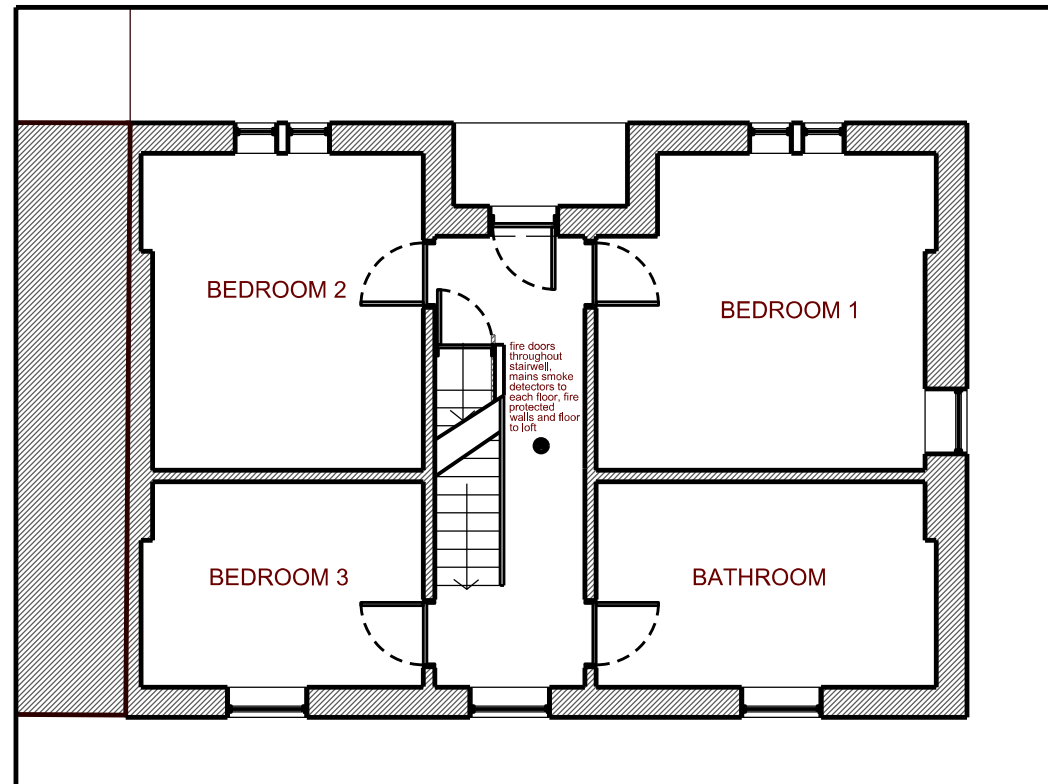
First Floor Plan - Proposed
