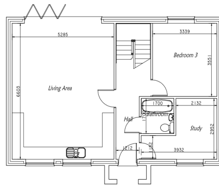
PROPOSED GROUND FLOOR LAYOUT
