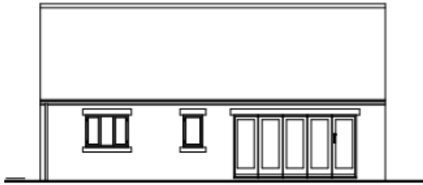
APPROVED REAR ELEVATION
