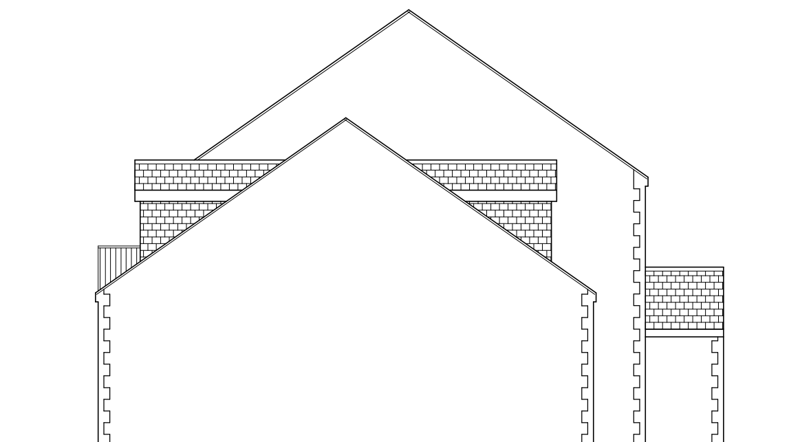
SIDE ELEVATION (GARAGE)
