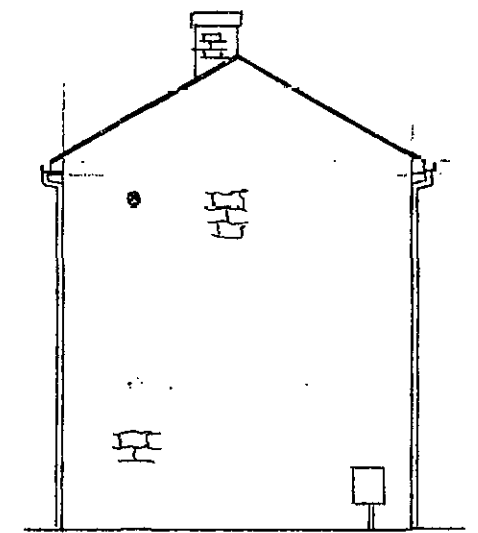
EXISTING GABLE ELEVATION
