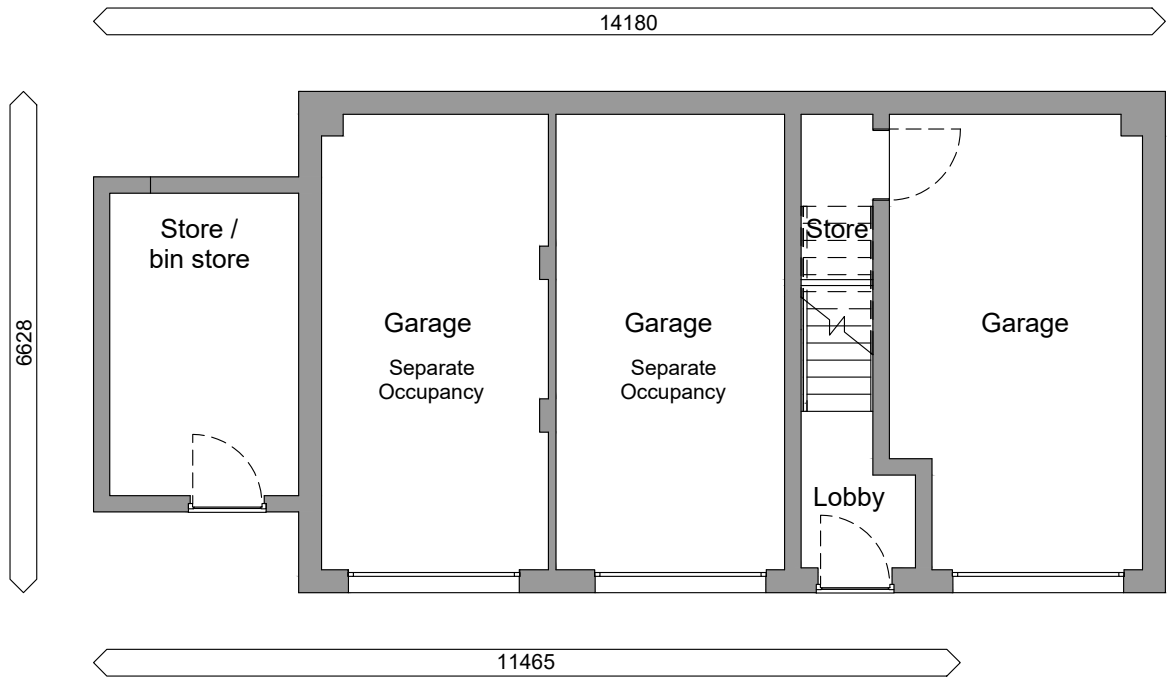
Ground Floor. 1 : 100
