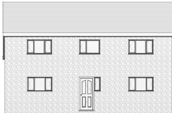
1 SOUTH EAST 1 : 100
