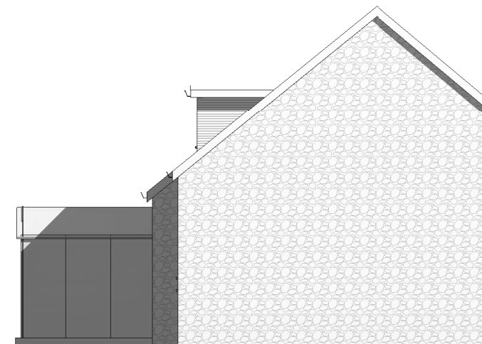
2 NORTH EAST 1 : 100
