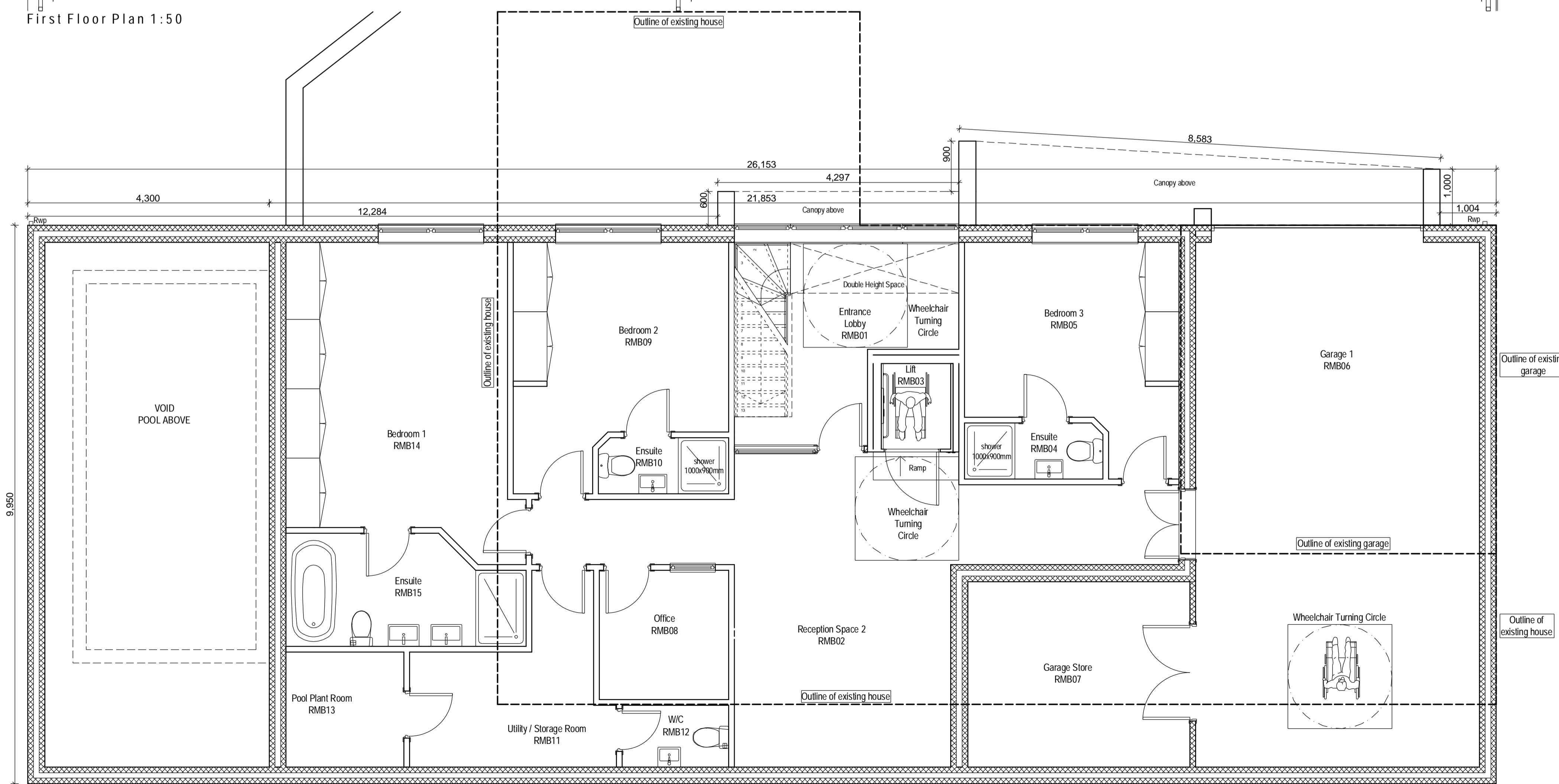
Ground Floor Plan 1:50
