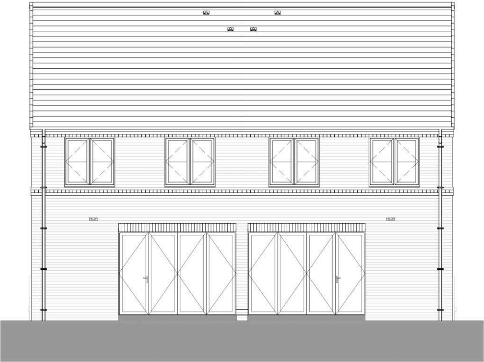
REAR ELEVATION HAMILTON
