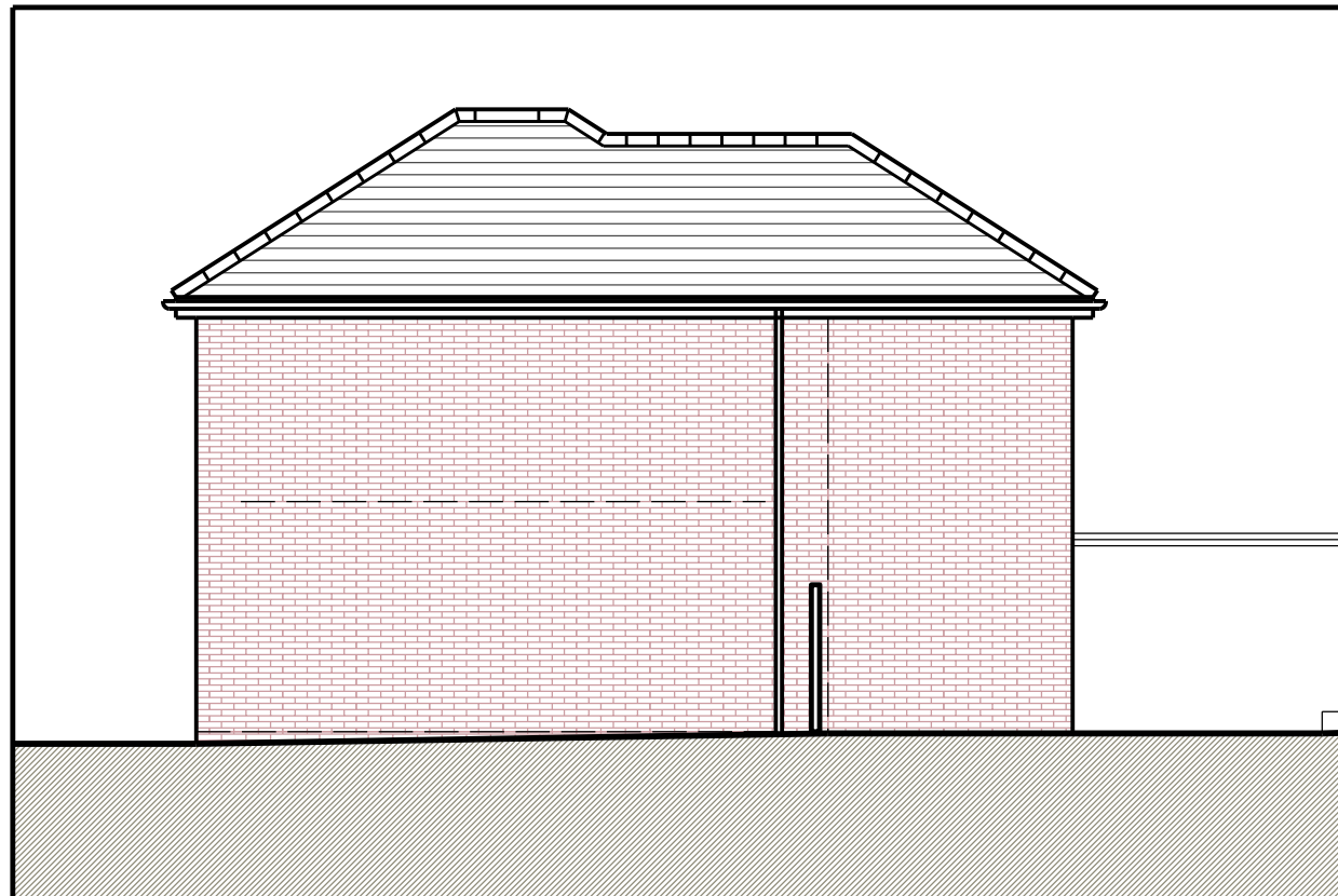
South Elevation
