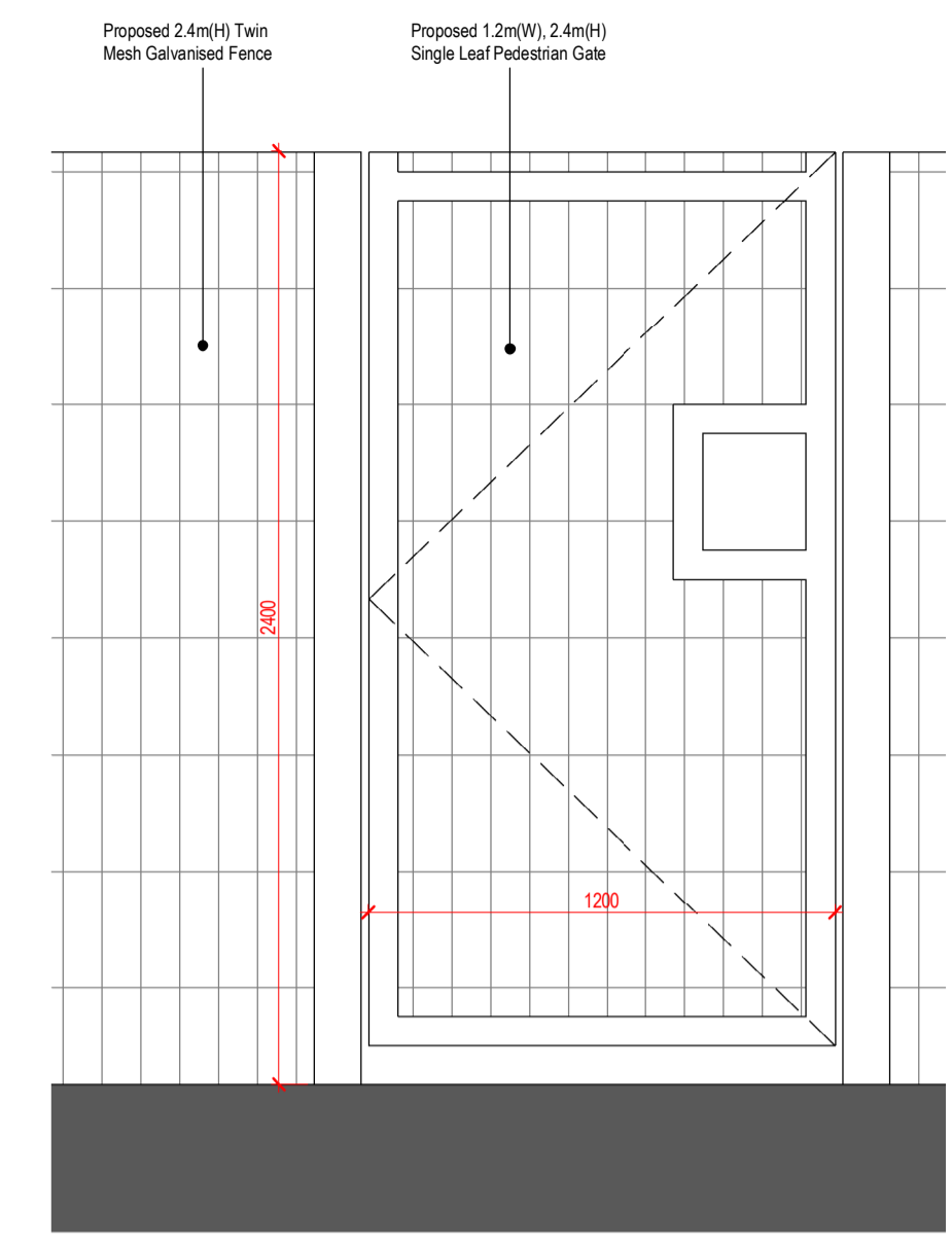
3 Typical Fence and Gate Elevation 1:20 Ref Sheet: 0002
