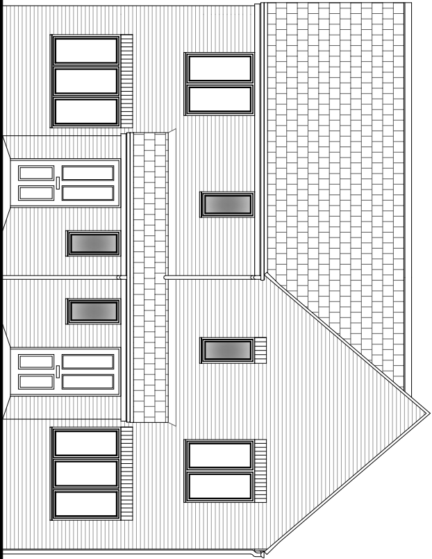
Front Elevation
