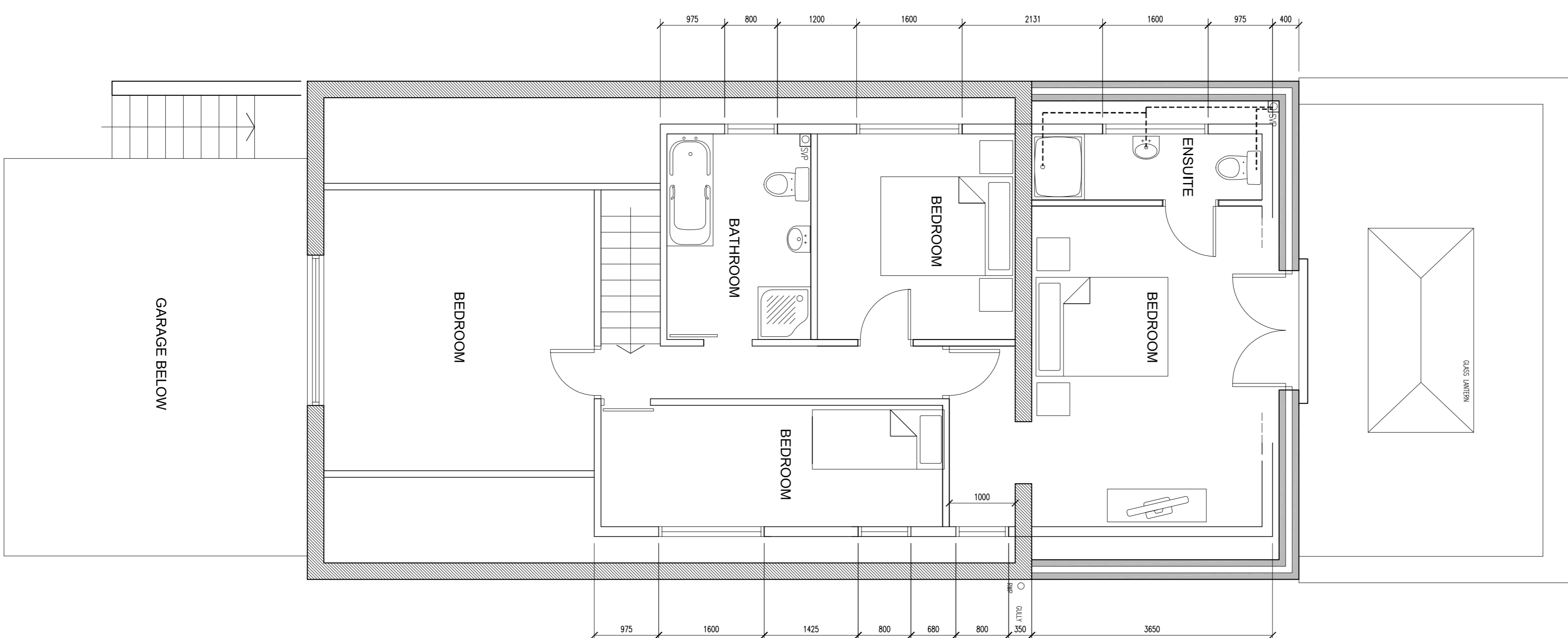
FIRST FLOOR
