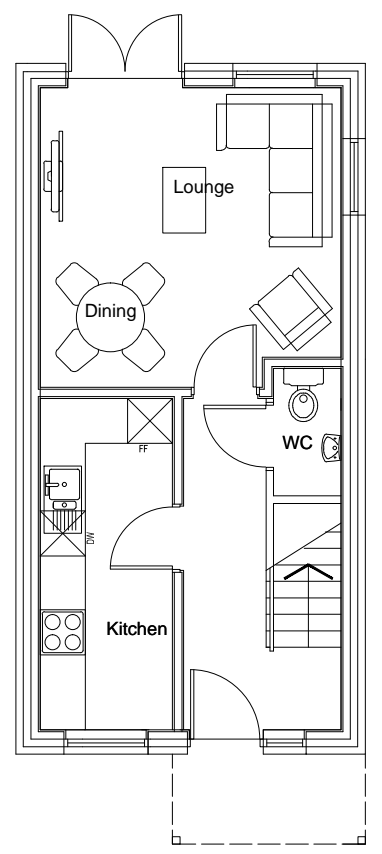
GROUND FLOOR PLAN AREA - 34sqm
