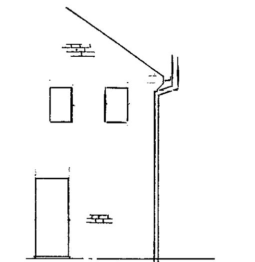
EXISTING REAR PART GABLE ELEVATION
