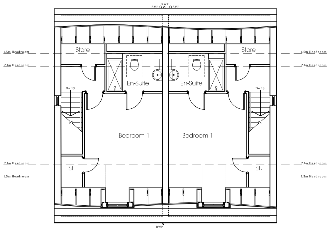
Second Floor Scale - 1:100
