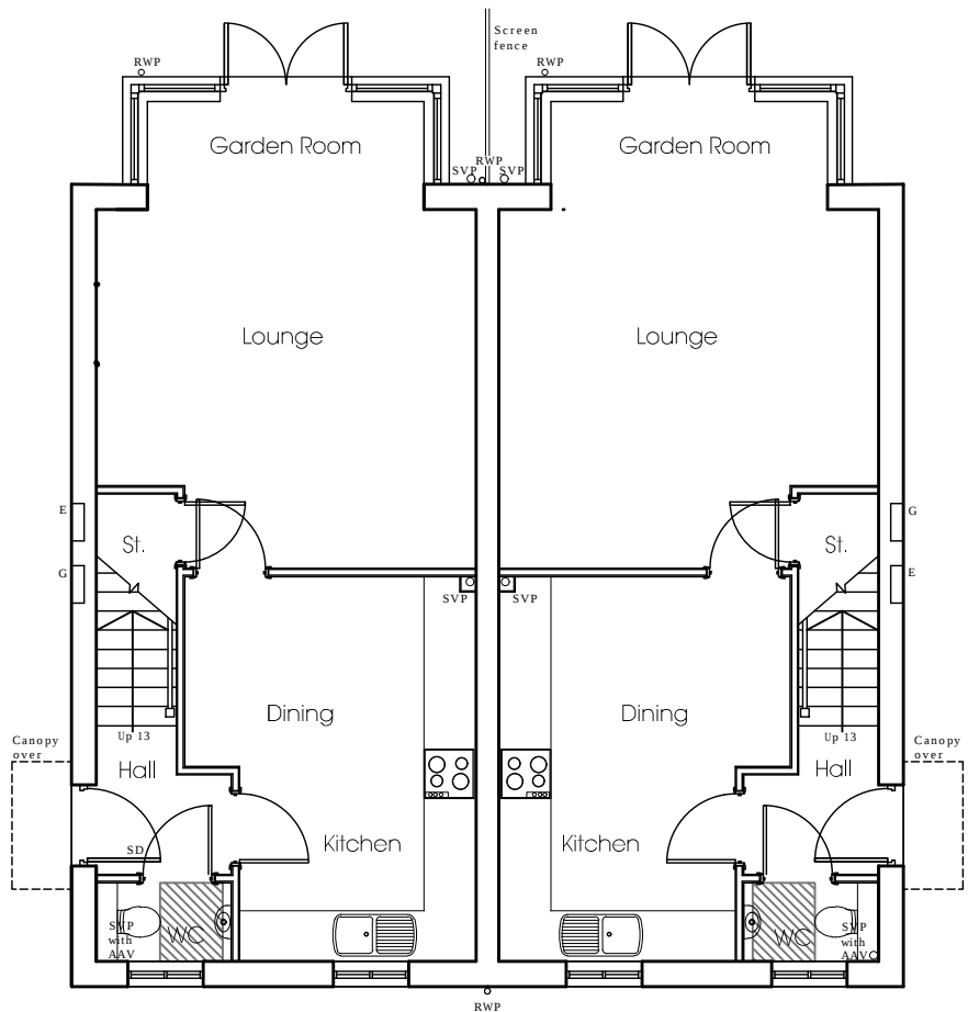
Ground Floor Scale - 1:100
