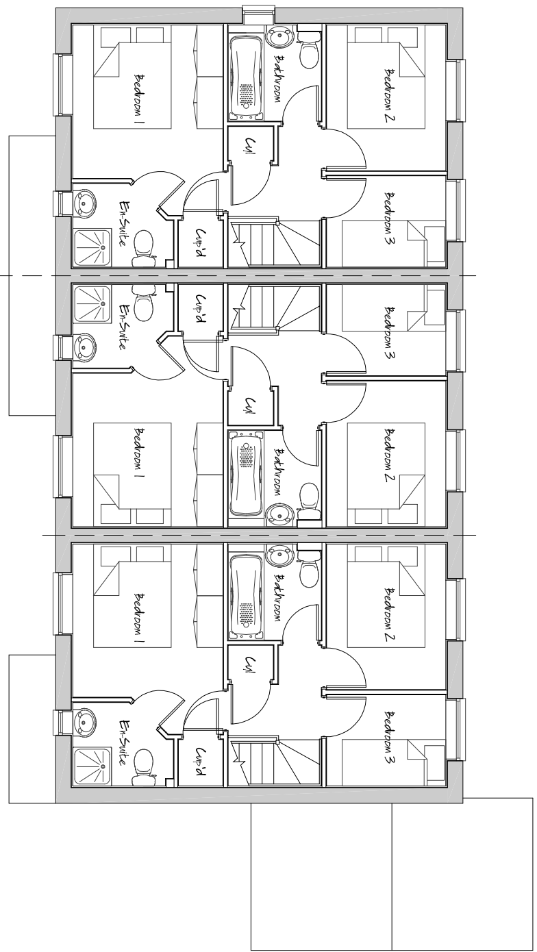
First Floor Layout
