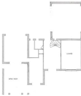
PROPOSED GROUND FLOOR LAYOUT
