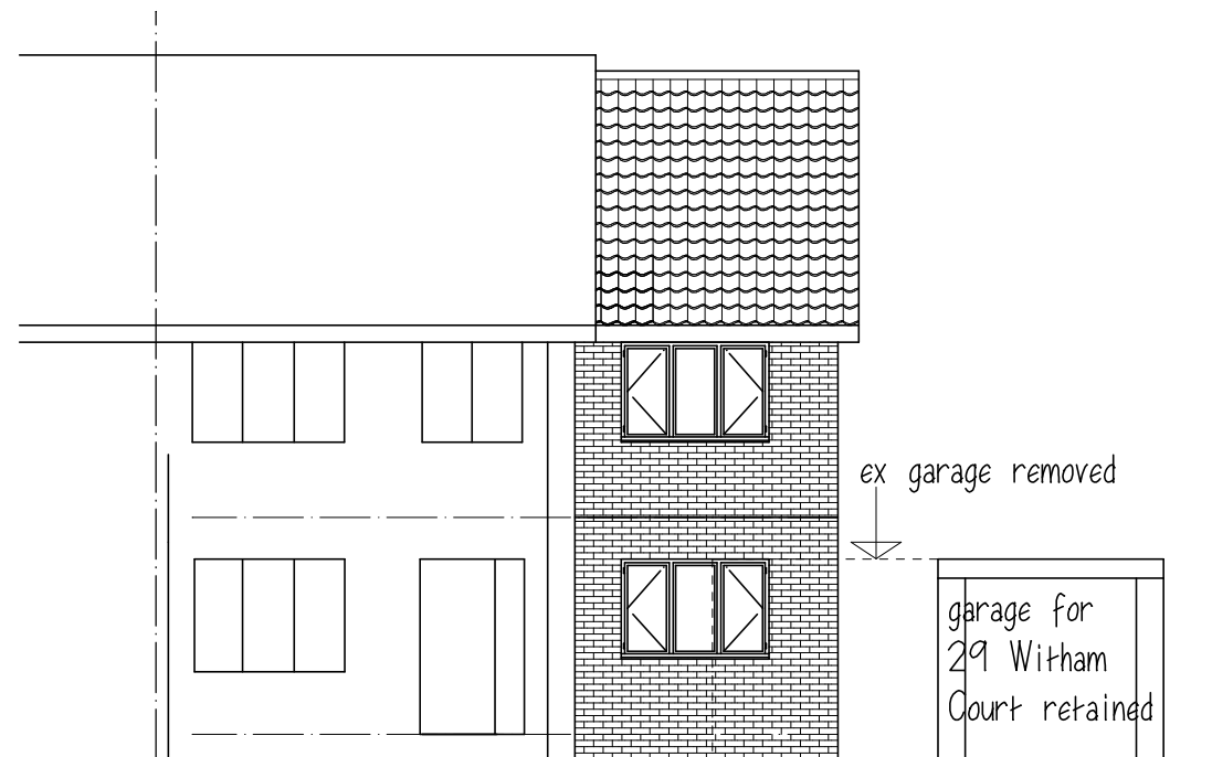
FRONT ELEVATION
