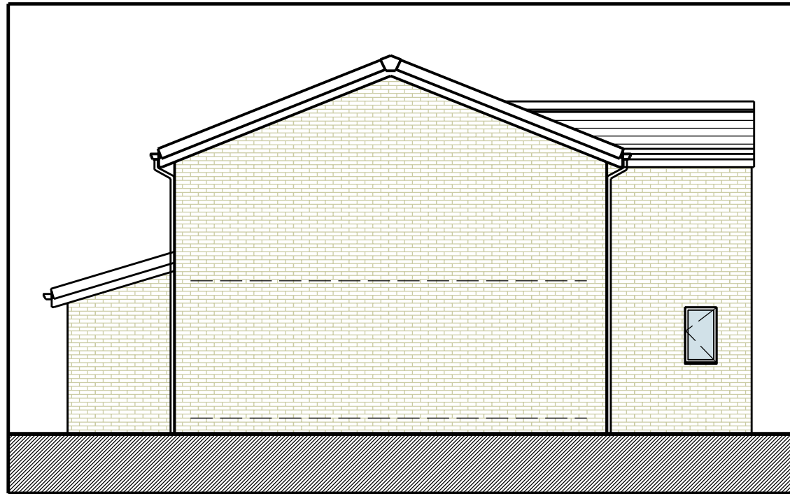
North Elevation
