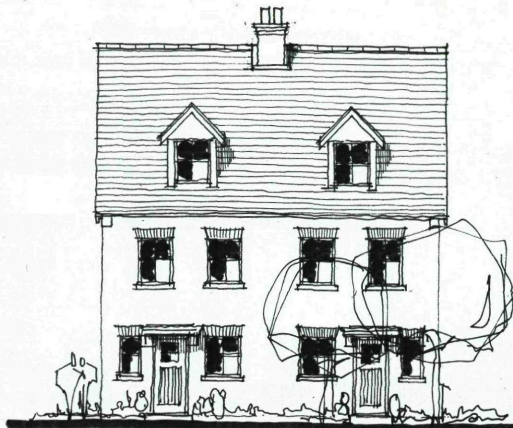
FRONT ELEVATION. 1:100.
