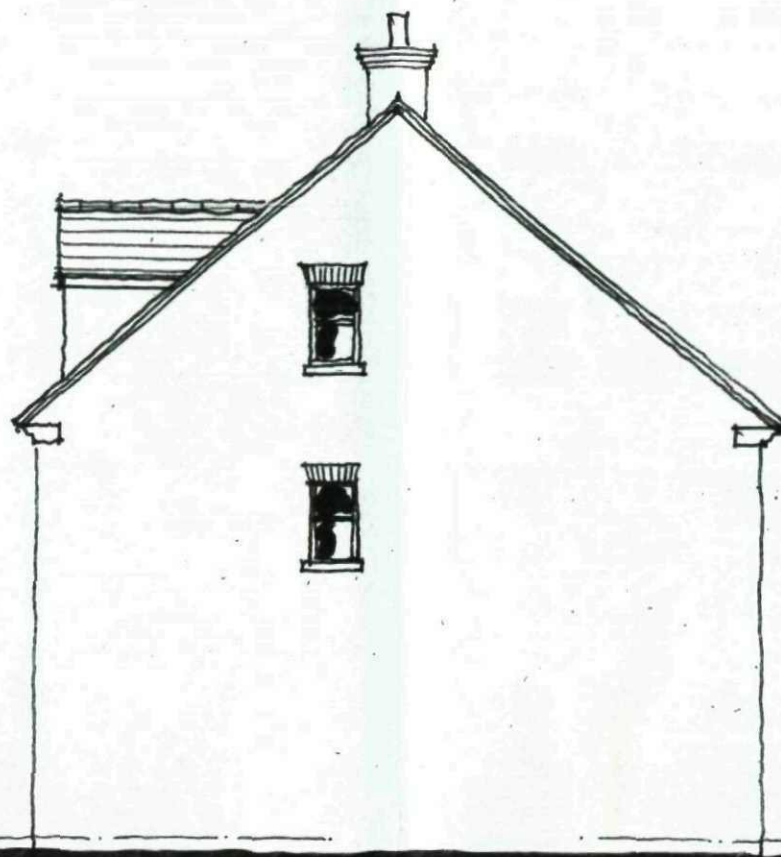
SIDE ELEVATION.
