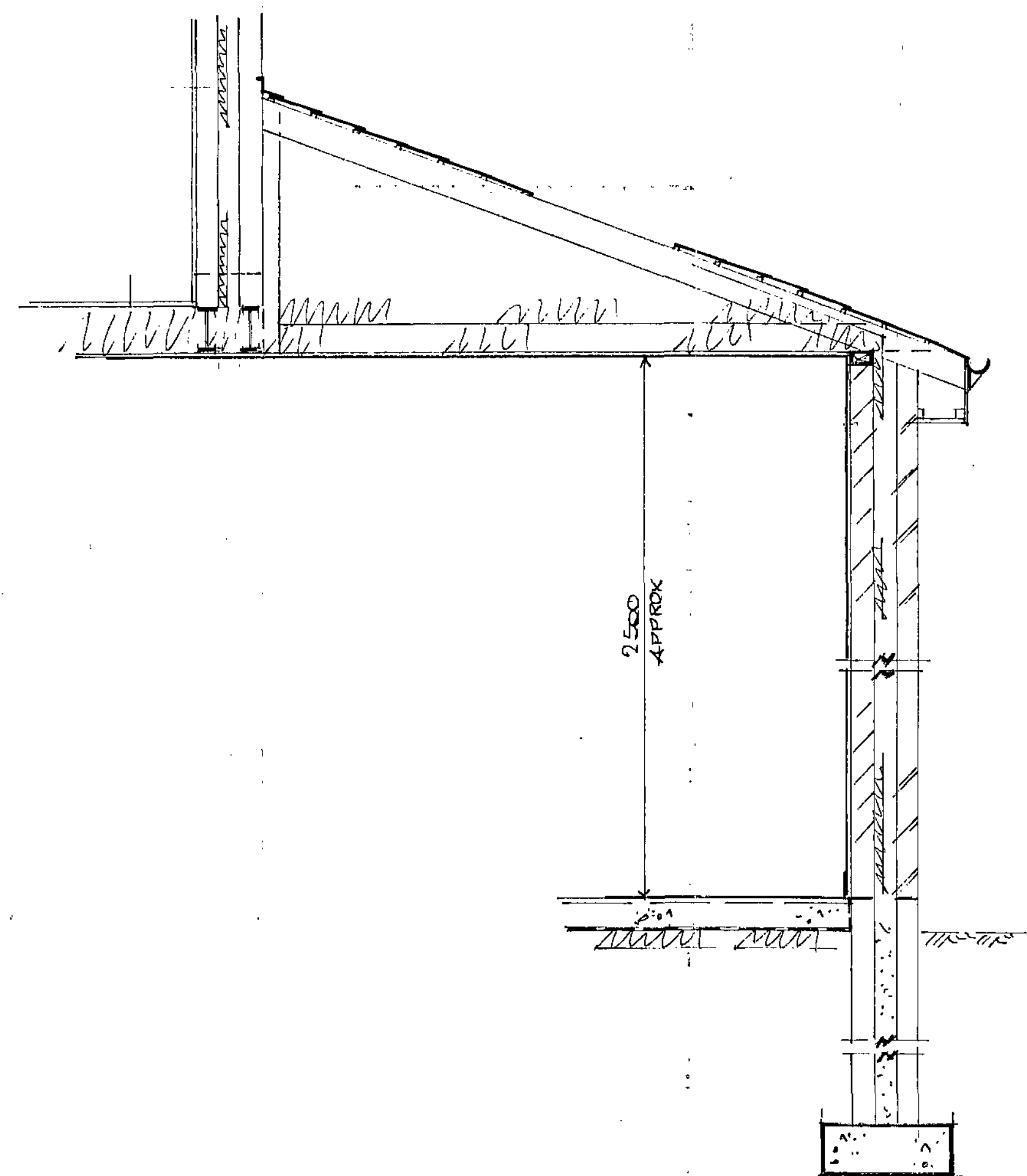
Typical Section on A - A
