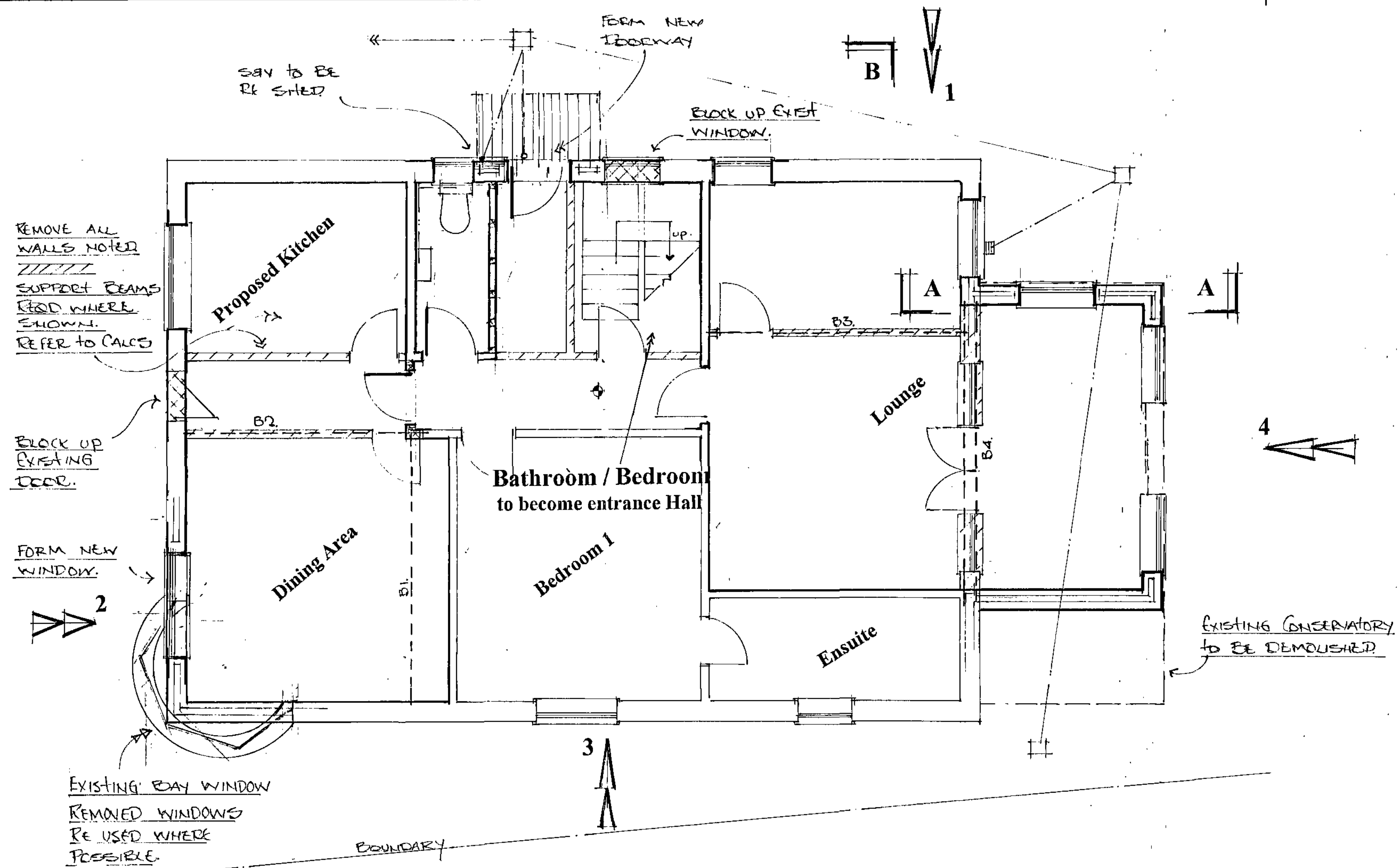
Existing / Proposed Ground Floor Layout
