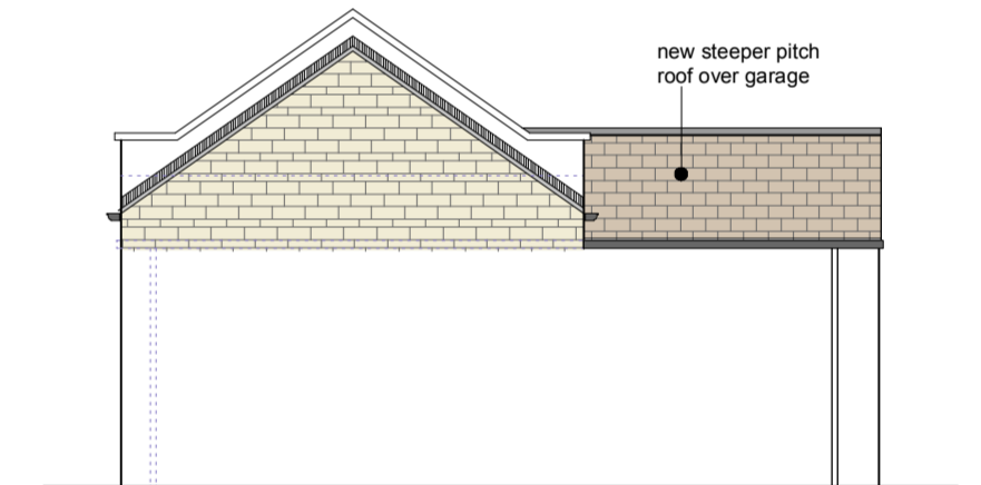
side elevation east
