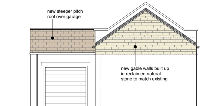
side elevation west
