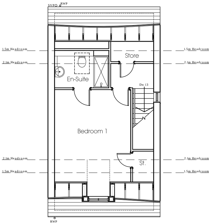
Second Floor Scale - 1:100
