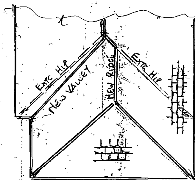
ROOF PLAN
