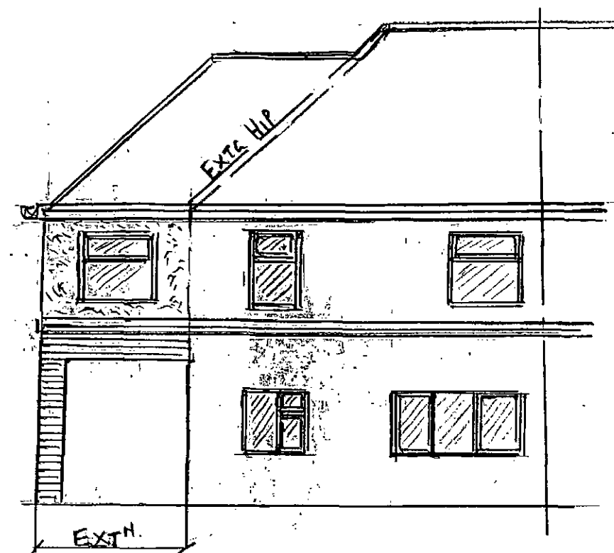
PROPOSED REAR ELEV N
