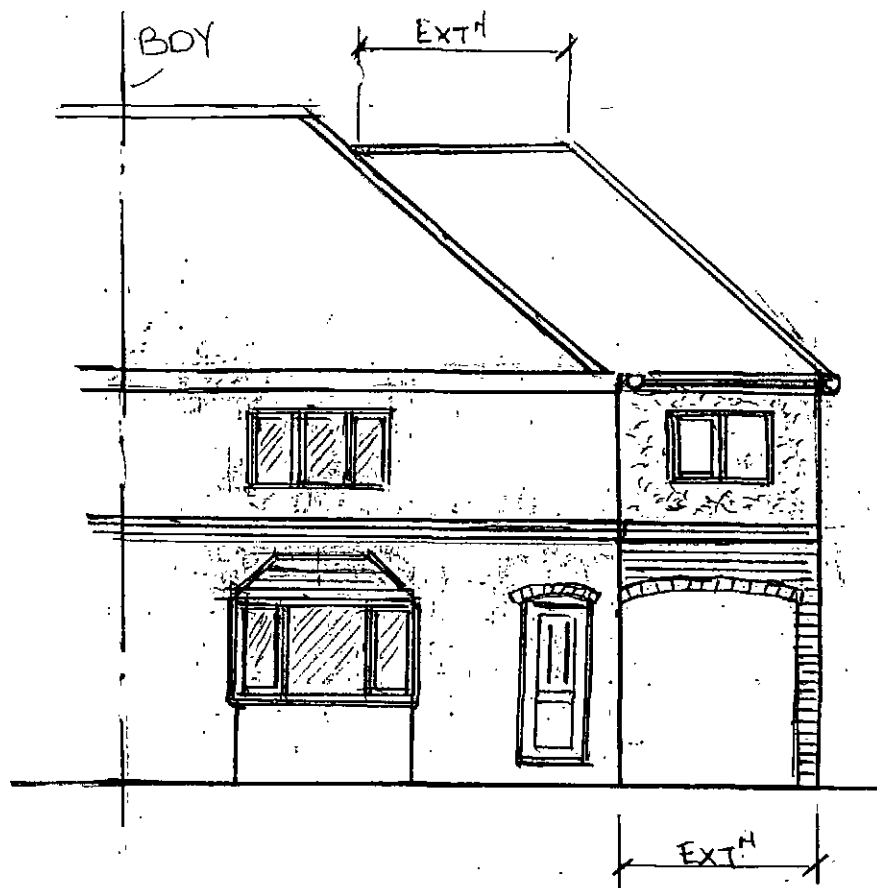
PROPOSED FRONT ELEV N
