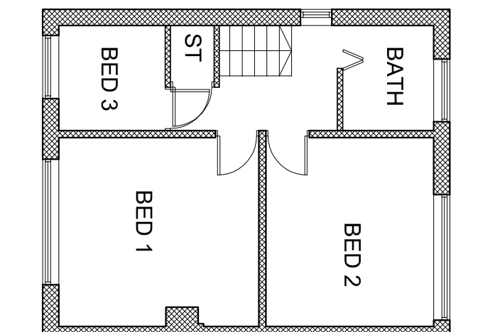
EXISTING FIRST FLOOR PLAN SCALE 1:100
