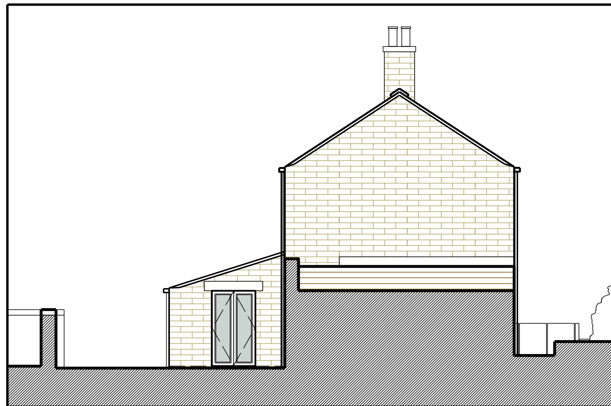
South Elevation
