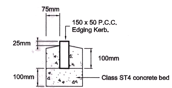
FOOTWAY EDGING DETAIL Scale 1:10
