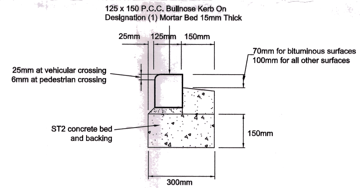
DRIVEWAY KERB DETAIL Scale 1:10
