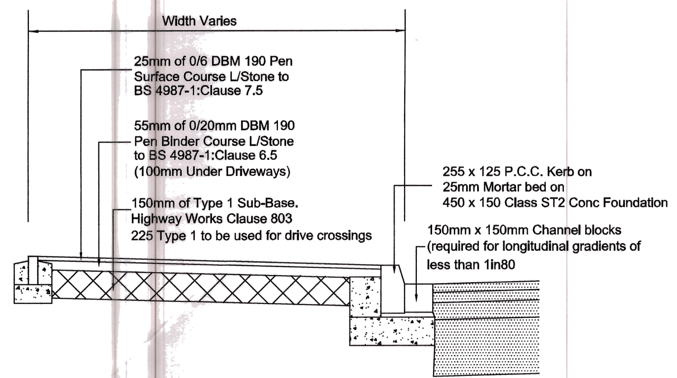
FOOTWAY RE-CONSTRUCTION Scale 1:20
