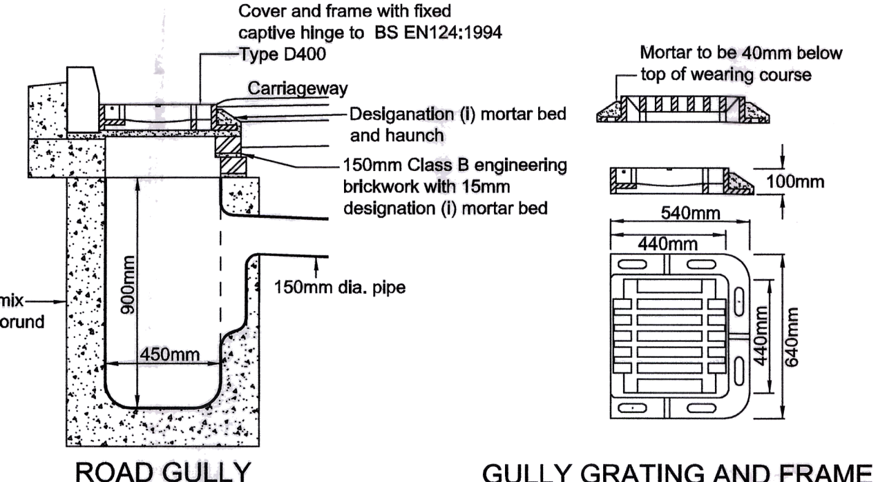
ROAD GULLY
