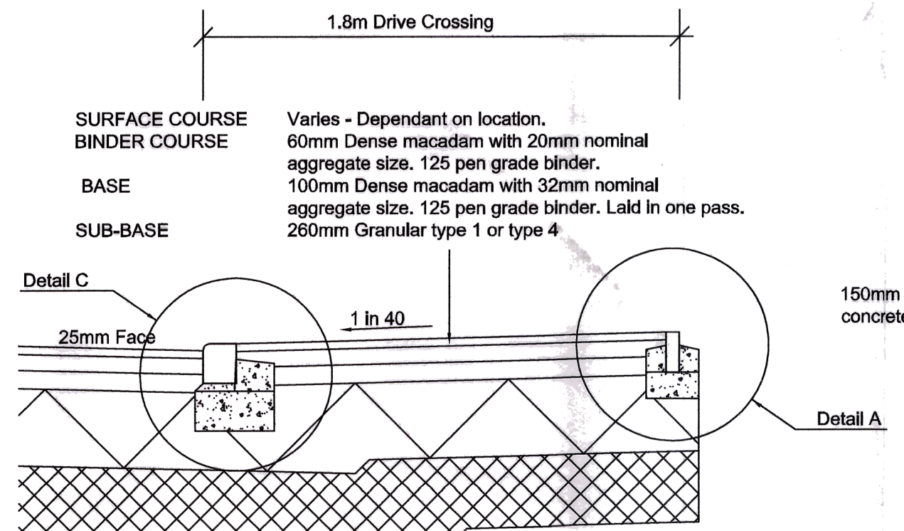
DRIVEWAY CROSSING DETAIL
