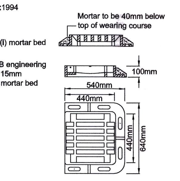
GULLY GRATING AND FRAME Scale 1:10
