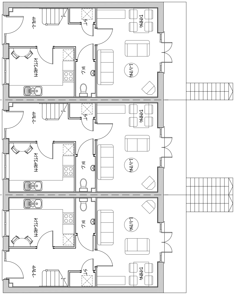
Ground Floor Layout
