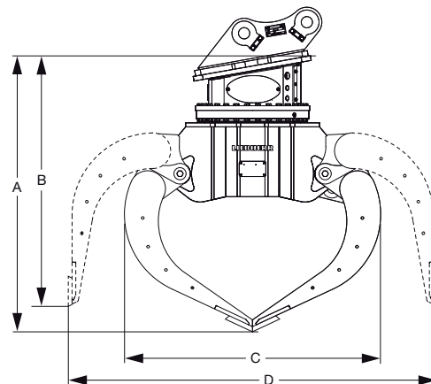
Rock grapple
