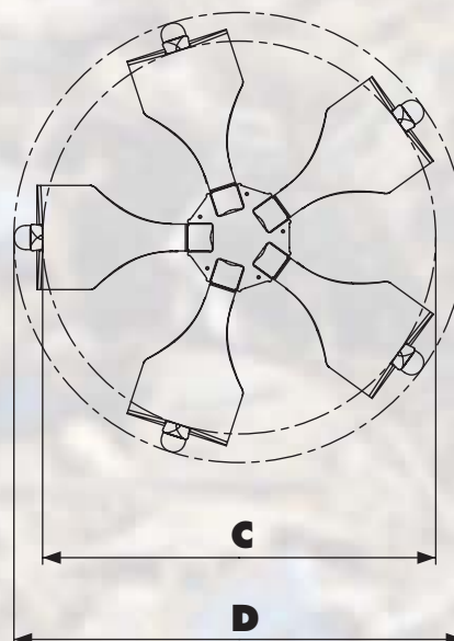
5-tine grapple, bottom view, closed
