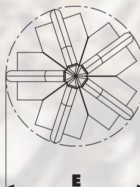
5-tine grapple, bottom view, closed
