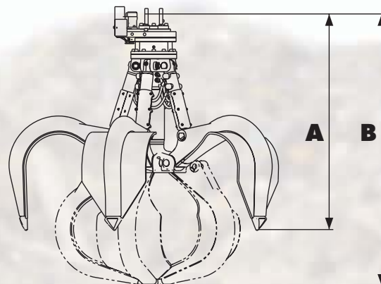
5-tine grapple, lateral view
