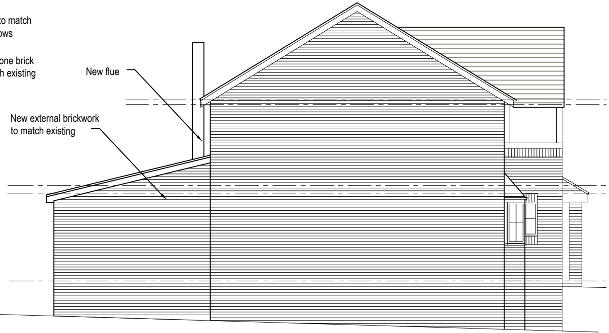
East Elevation
