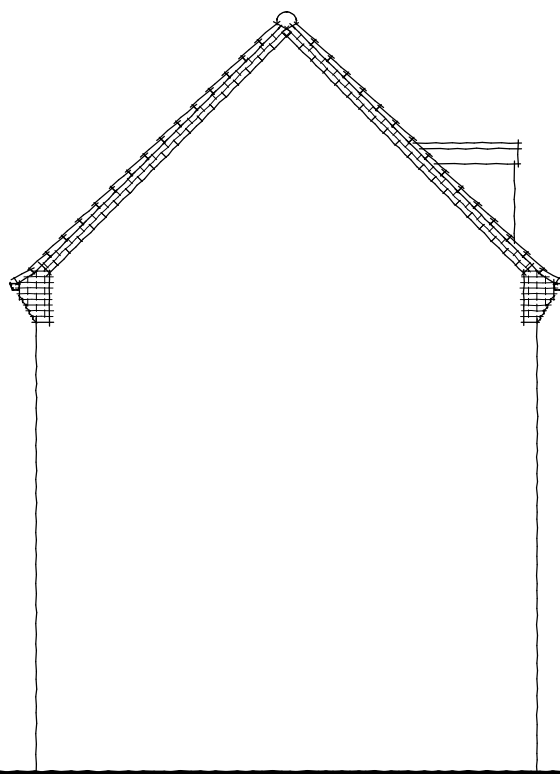
SIDE ELEVATION
