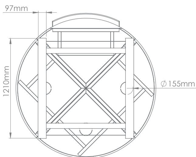
Bottom View
