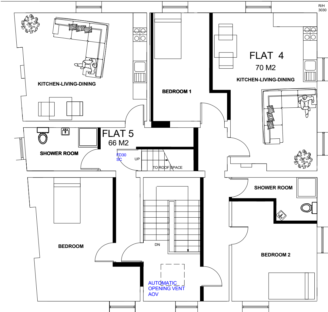
SECOND FLOOR
