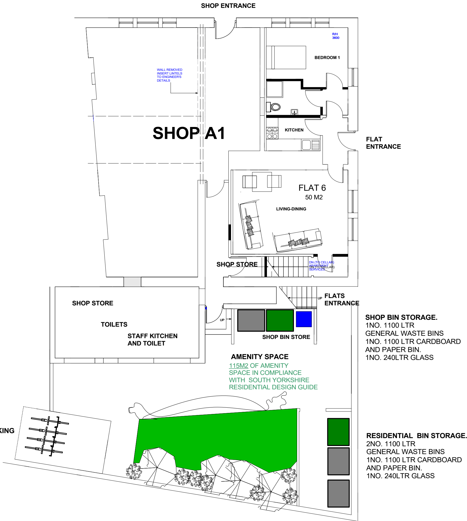
GROUND FLOOR
