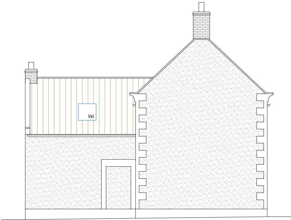
Existing Side Elevation @ 1:100 (A3)
