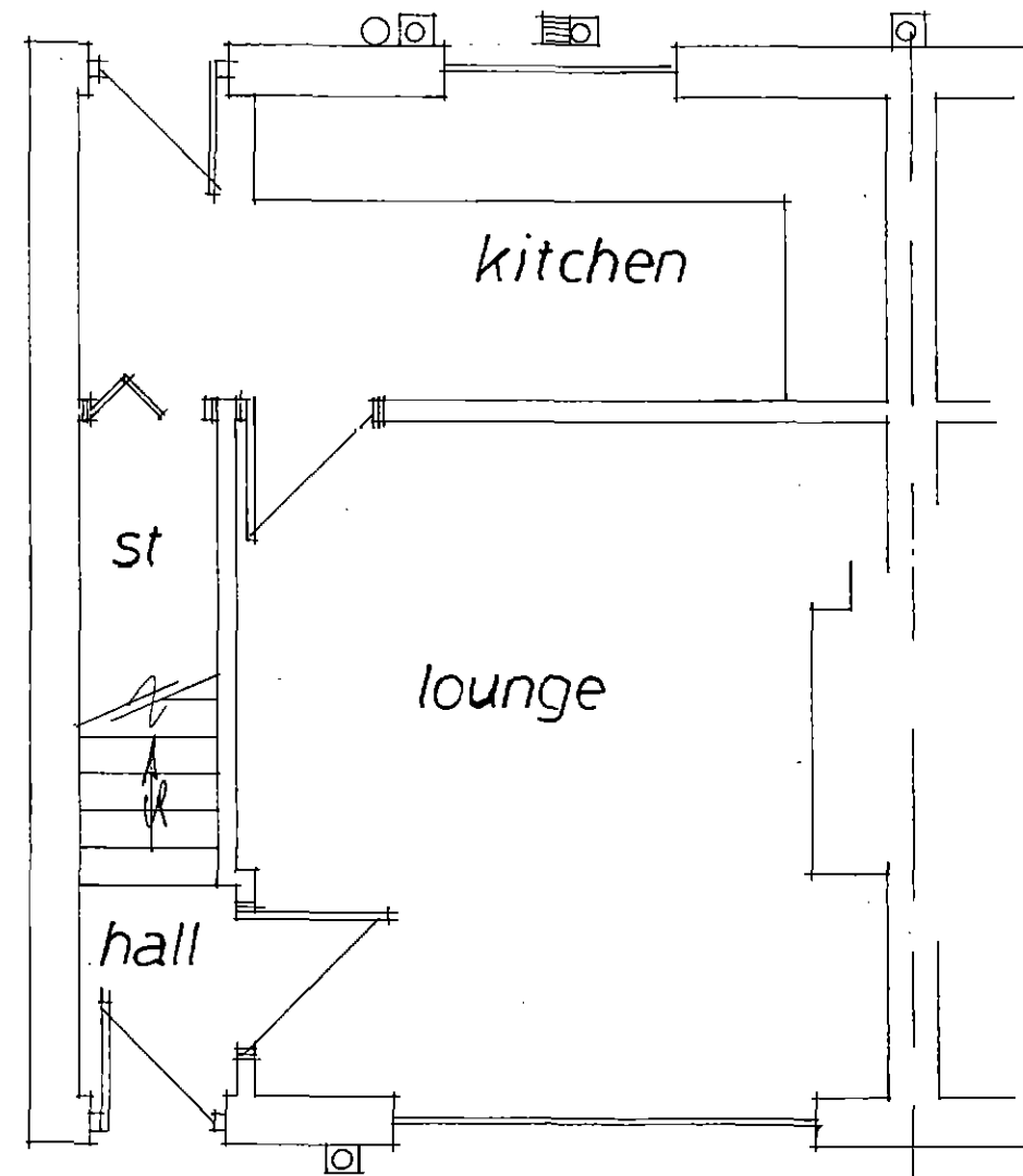
Ground Floor
