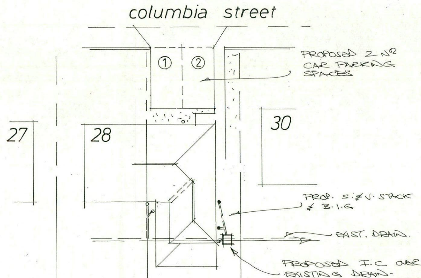
External Works Layout 1:200
