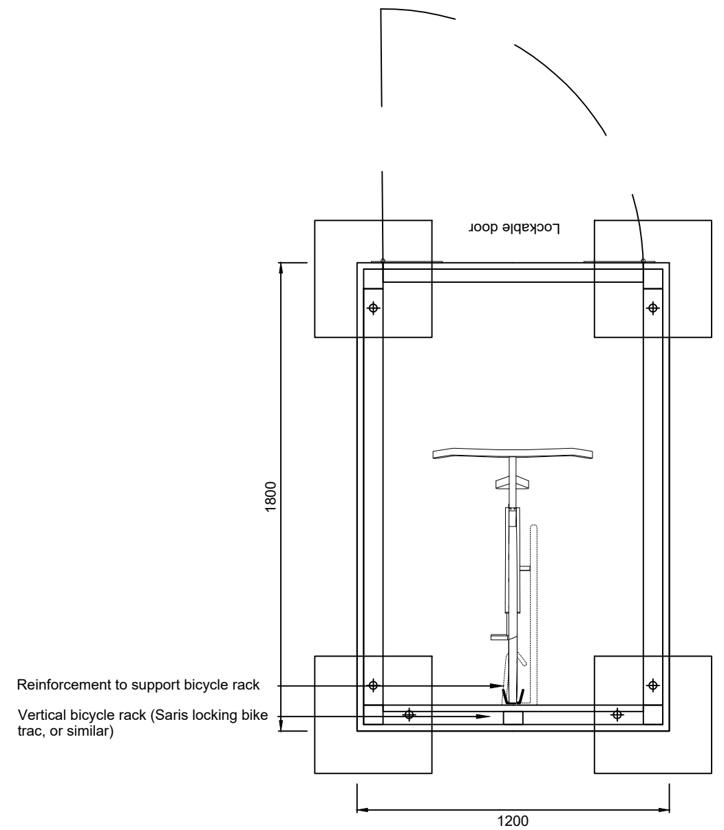
Cycle Store Plan
