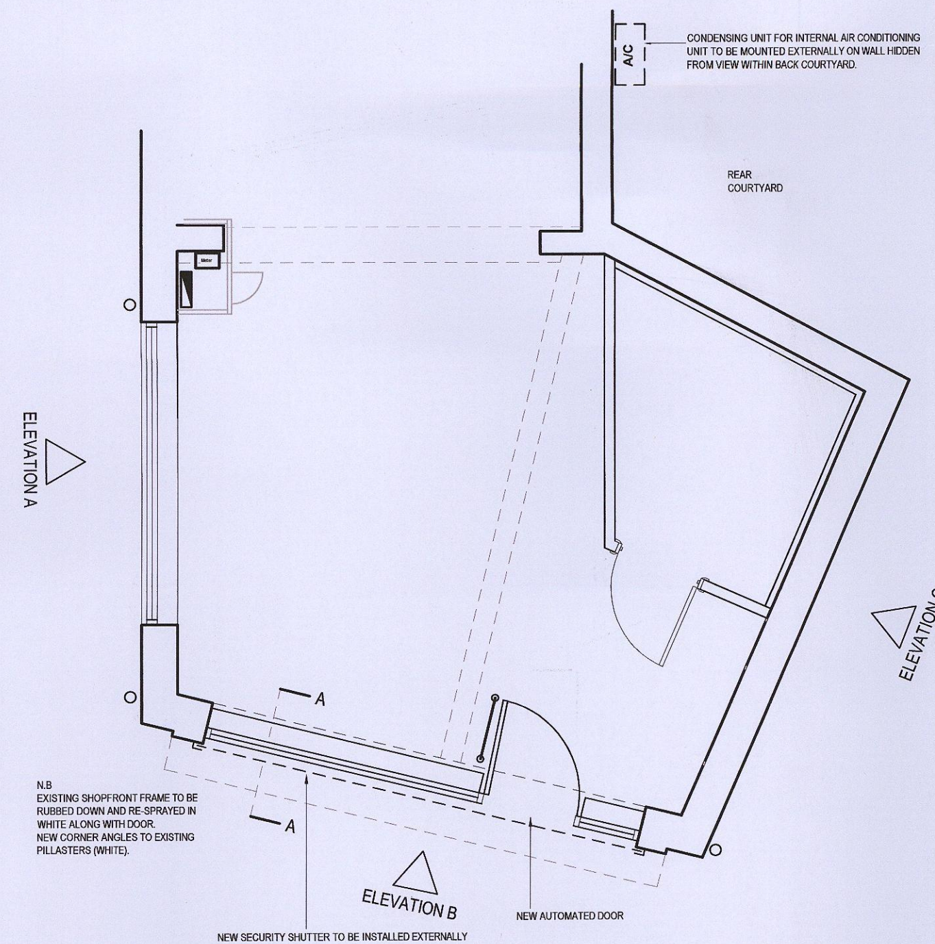
Proposed Plan 1:50
