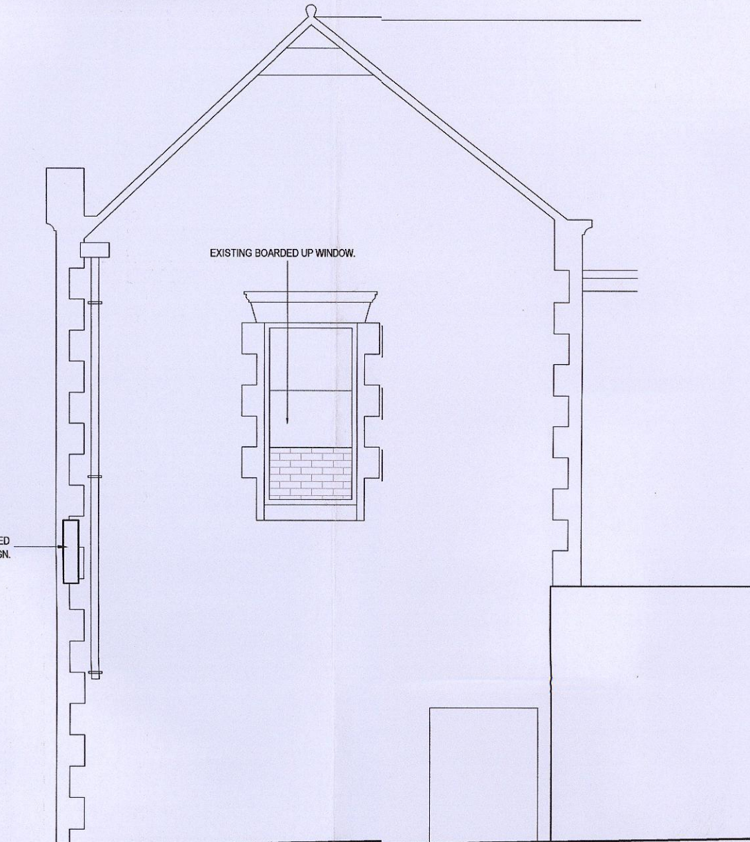
EXISTING ELEVATION C - 1:50
