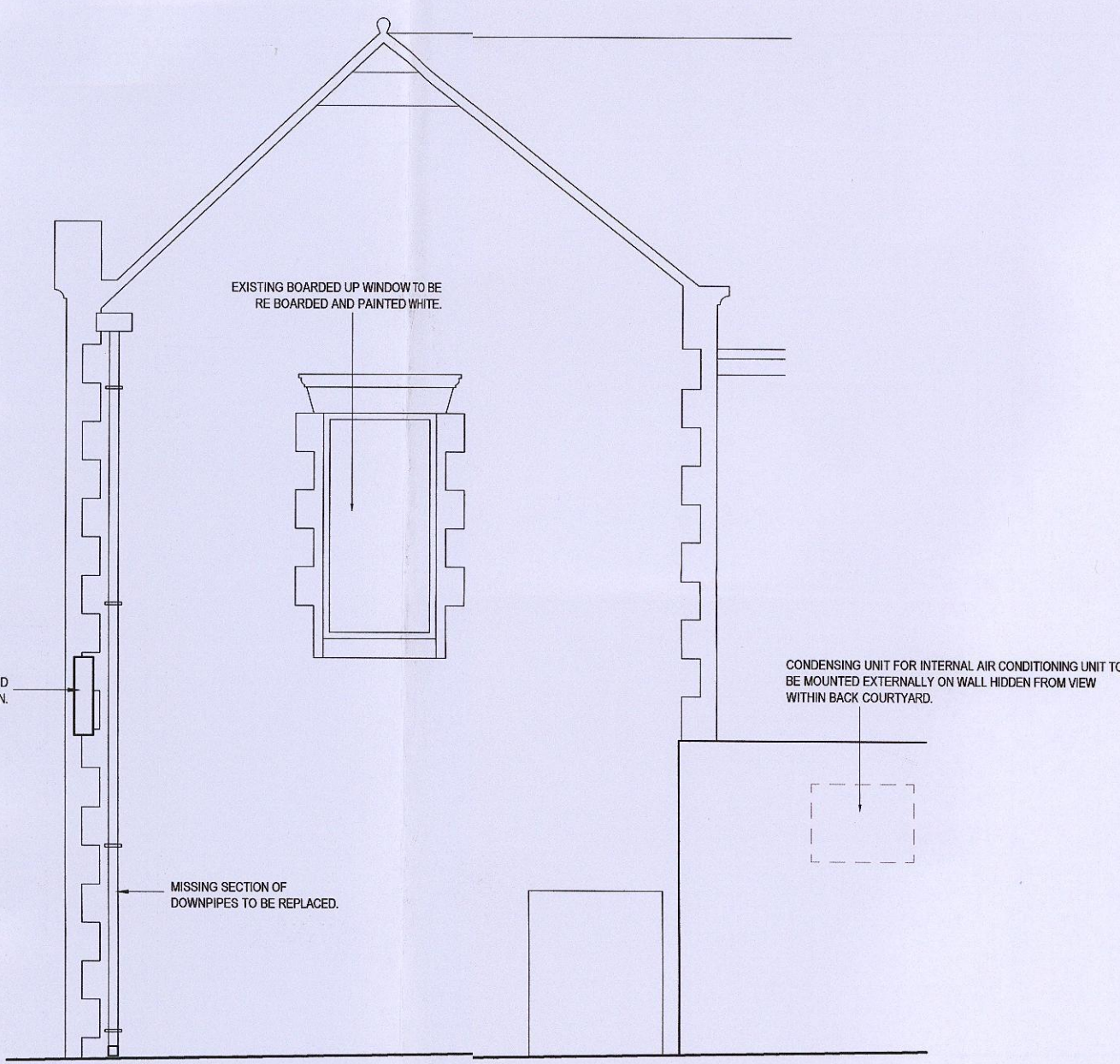
SECTION AA - 1:50
