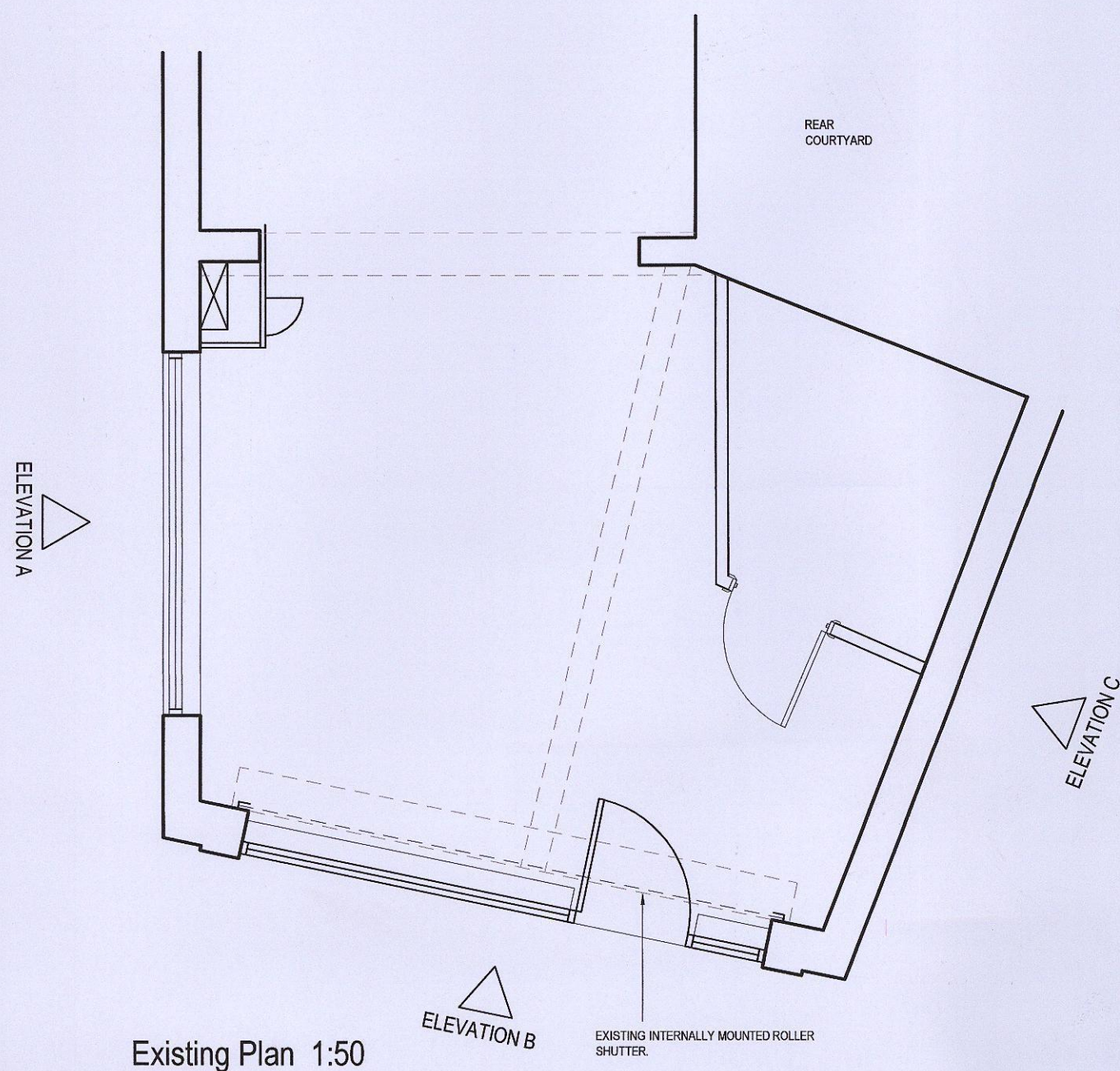
Existing Plan 1:50
