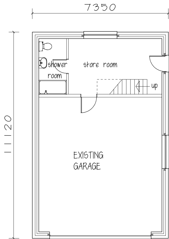
PLAN
